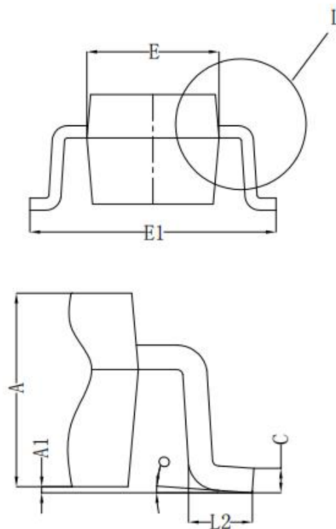
Detial L
